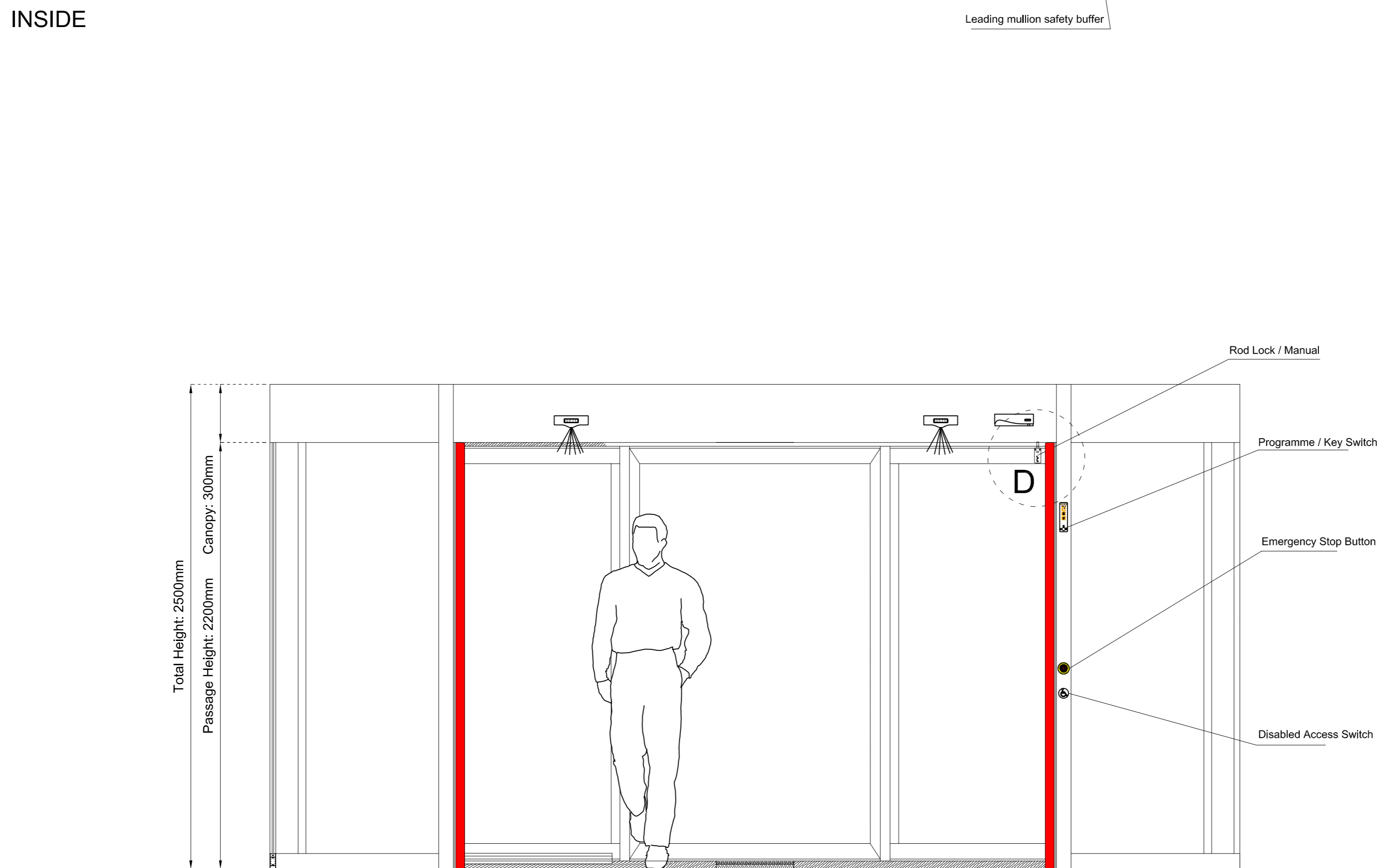
FRONT VIEW
