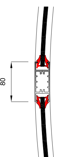
DETAIL C
